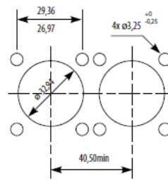
Square flange receptacle rear panel mounting
