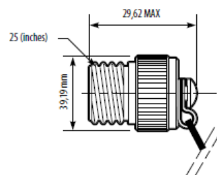
Protective cap for receptacles (nylon cord)
