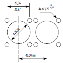
Square flange receptacle front panel mounting
