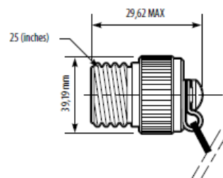
Protective cap for receptacles (nylon cord)
