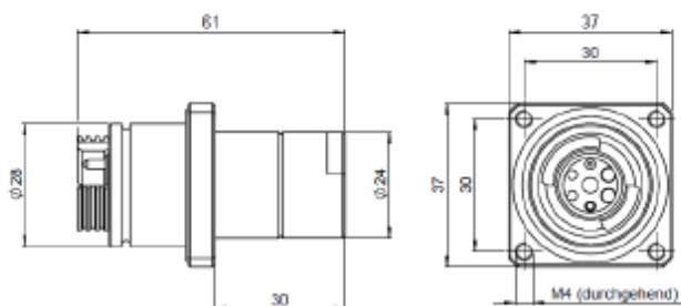
Flange Mount Receptacle
