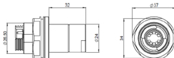
Jam Nut Mount Receptacle
